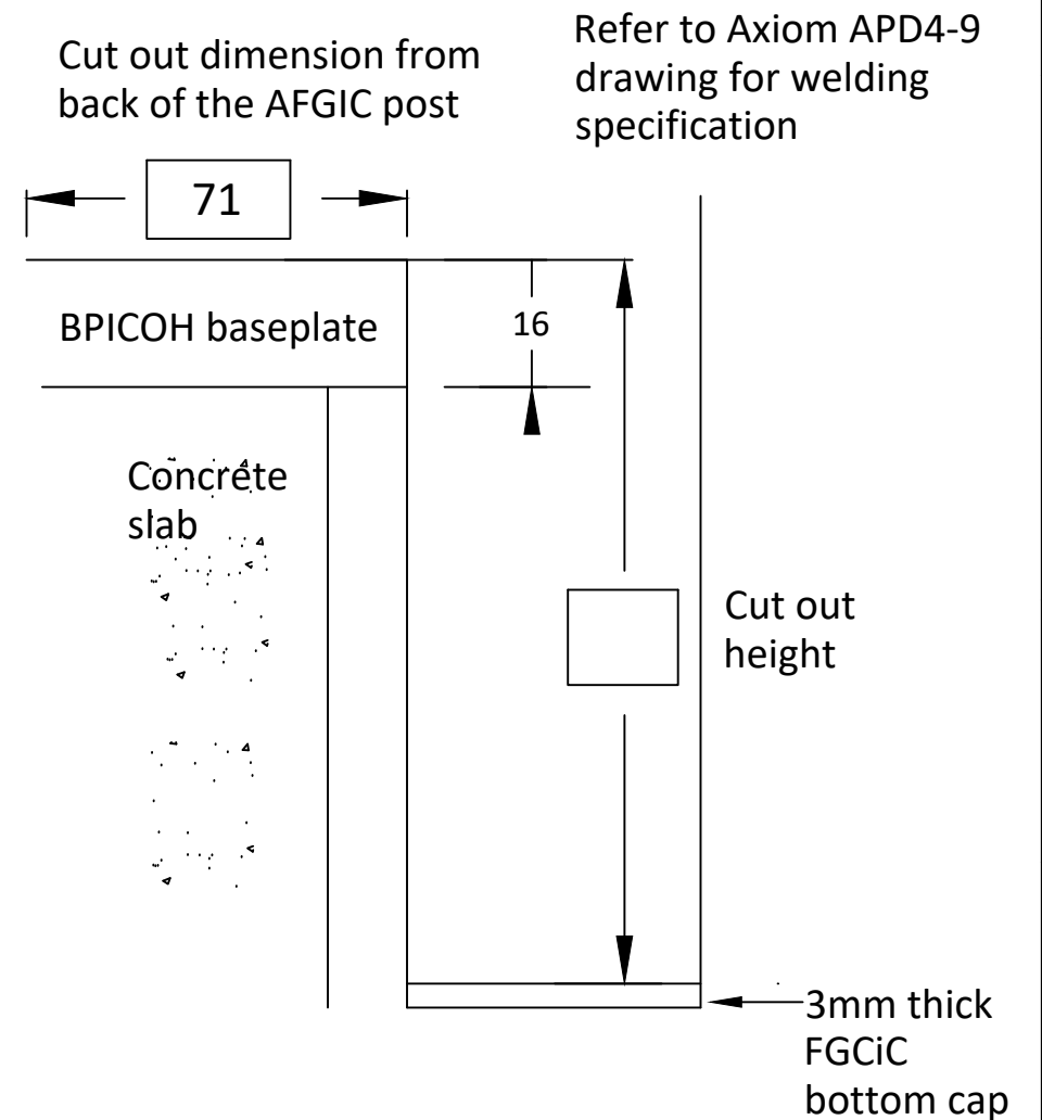
Side view cut detail of the AFGIC post and BPICOH baseplate connection
