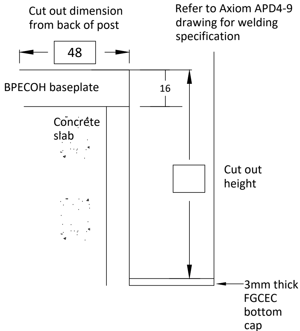
Side view cut detail of the AFGEC post and BPECOH baseplate connection
