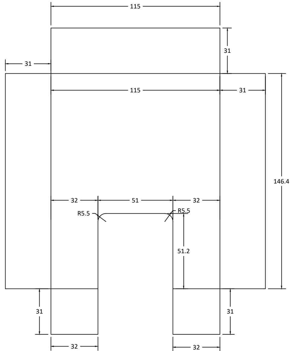
Plan view
