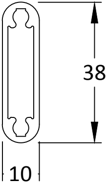
Axiom product code: AS-38 38x10mm slat.
